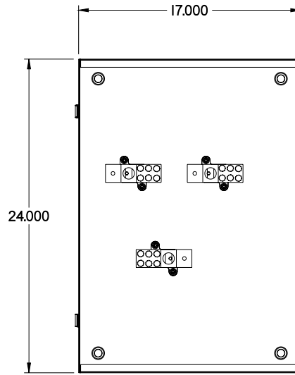
FRONT VIEW - COVER REMOVED
