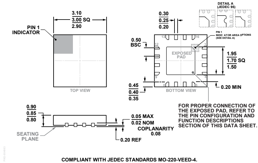
Figure 34. 16-Lead Lead Frame Chip Scale Package [LFCSP] 3 mm × 3 mm Body and 0.85 mm Package Height (HCP-16-1)
