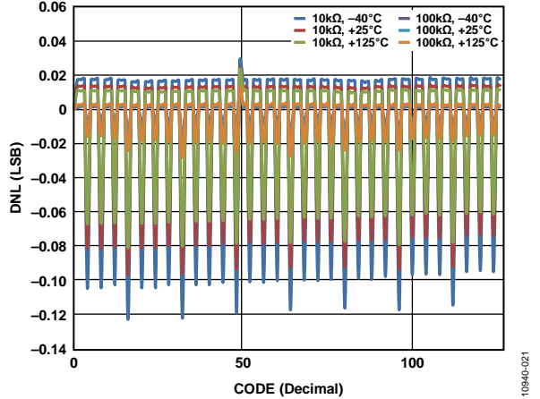
Figure 18. DNL vs. Code (AD5121)
