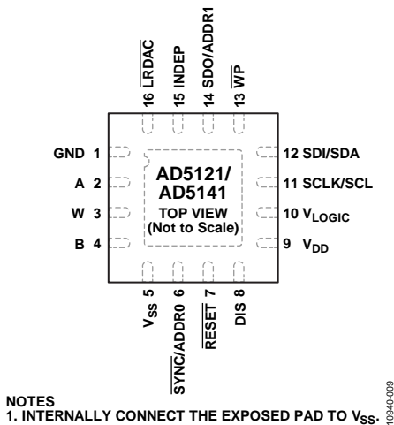
Figure 7. Pin Configuration
