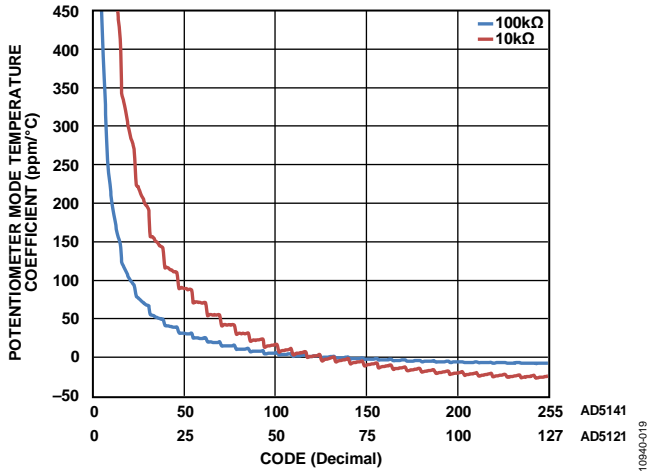
Figure 15. Potentiometer Mode Temperature Coefficient ((\Delta V_{IW}/V_{IW})/\Delta T \times 10^6) vs. Code
