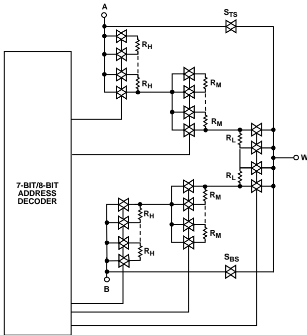
Figure 42. AD5121/AD5141 Simplified RDAC Circuit
