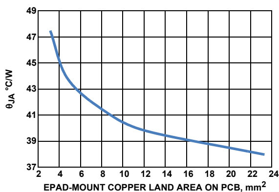
FIGURE 29. 3mmx3mm-10 PIN DFN ON 4-LAYER PCB WITH THERMAL VIAS \theta_{JA} vs EPAD-MOUNT COPPER LAND AREA ON PCB
