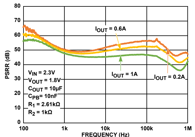
FIGURE 2. PSRR
