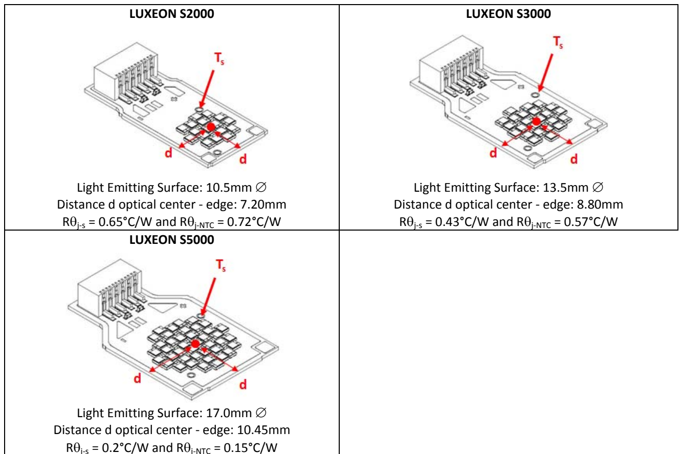
Figure 1. Mechanical and thermal characteristics for each LUXEON S emitter configuration. This information is applicable for both connector and connector-less versions.
