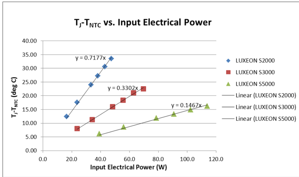
Figure 10. This graph shows the linear relationship between the device Junction Temperature, NTC Temperature and Input Electrical Power of the 3 LUXEON S devices.
