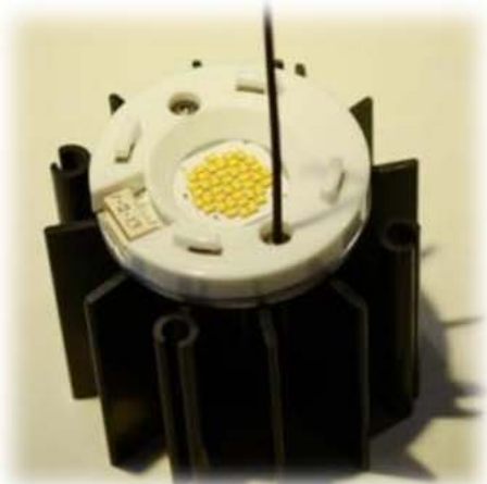
Figure 7. Suggested assembly procedure for LUXEON S5000 with an alternative clamping system, which can accommodate a reflector.
