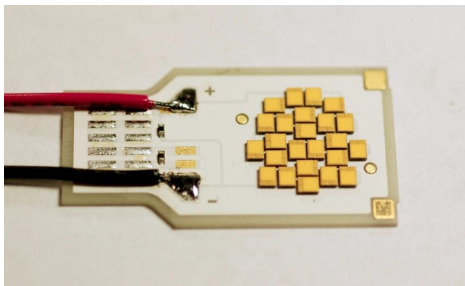
Figure 8. Example of a LUXEON S3000N with wires soldered to the anode and cathode pads.
