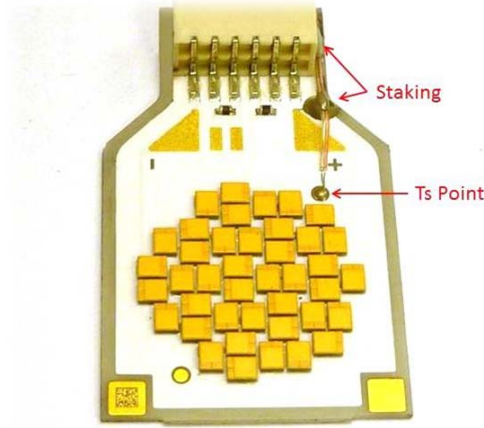
Figure 9. Picture of a properly mounted thermocouple on the circular T_s pad between the LEDs and the connector of a LUXEON S5000 emitter. The thermocouple is staked with additional silver epoxy at several points to keep it in place.
