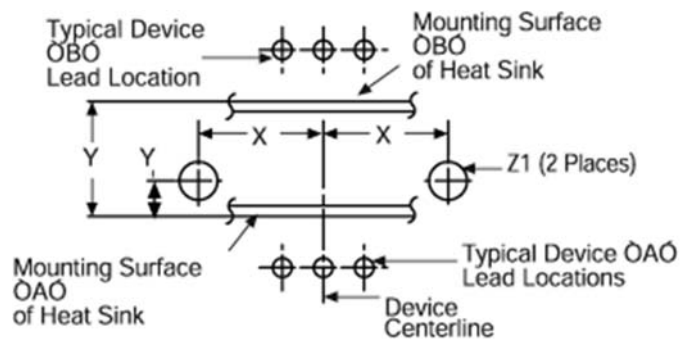
Mounting Details:
