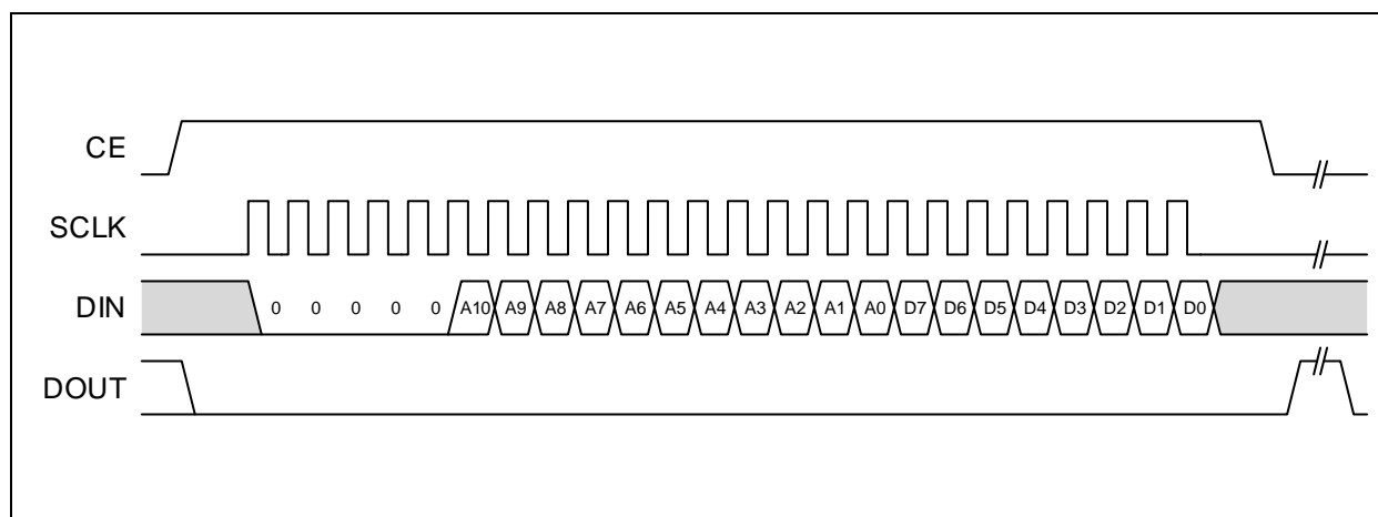
Figure 51: One-Byte Write
