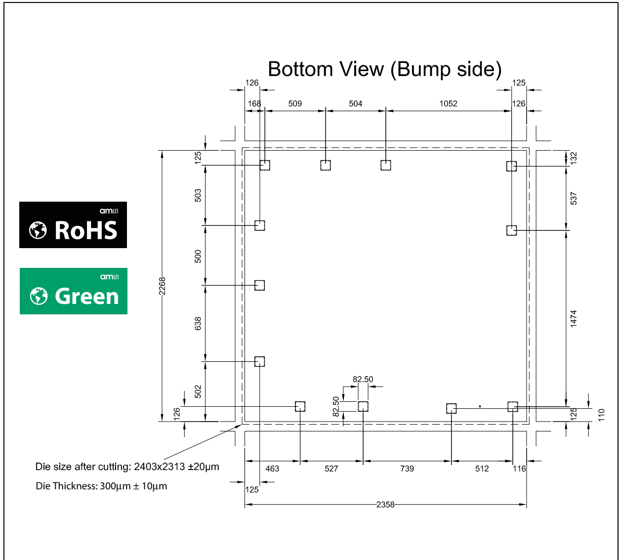
Figure 66: Package Outline Drawings Gold-Bumped Die (SW)
