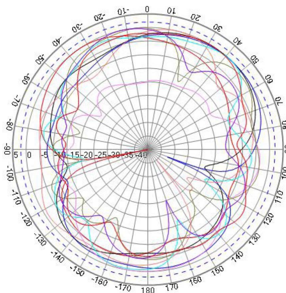
XZ PLANE
