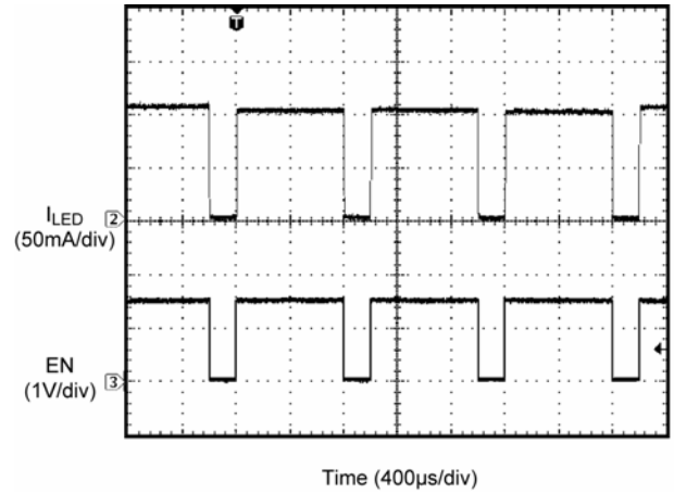
Figure 9. PWM Signal at 80% Duty Cycle ( I_{avg} = 80\text{mA} )
