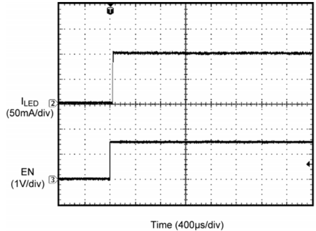
Figure 10. PWM Signal at 100% Duty Cycle ( I_{avg} = 100\text{mA} )
