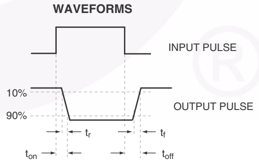
Figure 12. Switching Time Test Circuit and Waveforms
